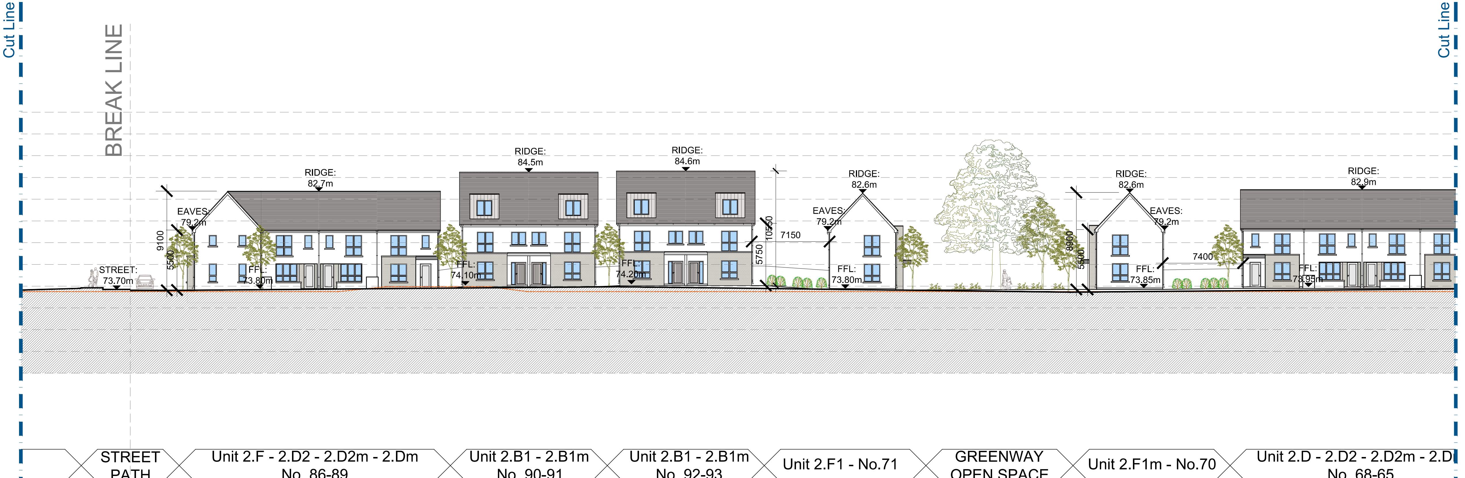
PROPOSED SITE SECTION CC (Zoom 3) - scale 1:200
